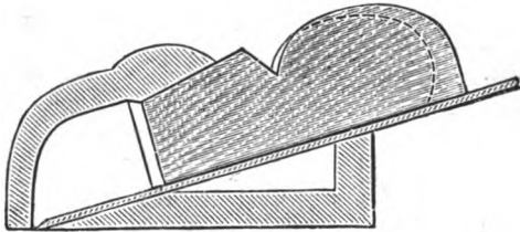
Fig. 8.—Bull-nose Plane in Section.
