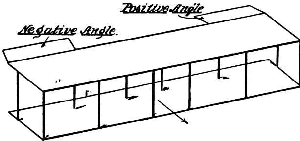
Farman Ailerons. Fig. 49.
