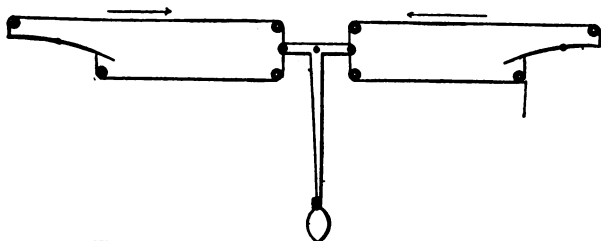
Fig. 68. Pendulum Stabilizers.
