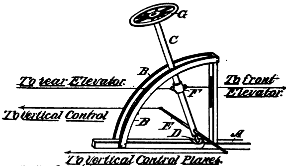
Fig. 69. Steering and Control Wheel.
