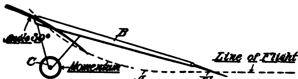
Fig. 20. Action when Propeller ceases to pull
