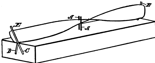
Fig. 88. Making the Propellor.
