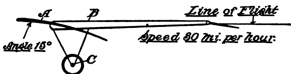
Fig. 19. Normal flight, with Propeller pulling.
