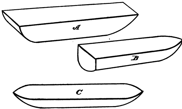
Fig. 75. Hydroplane Floats.
