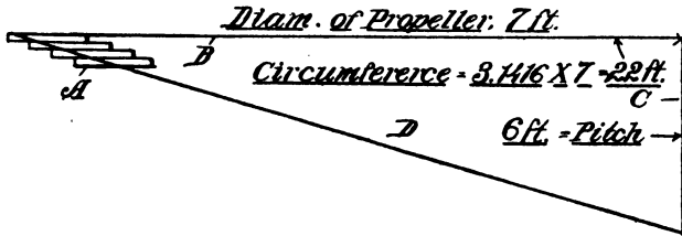
Fig. 77. Laying out the Pitch.
